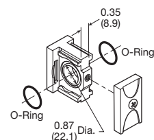
Body Connector
