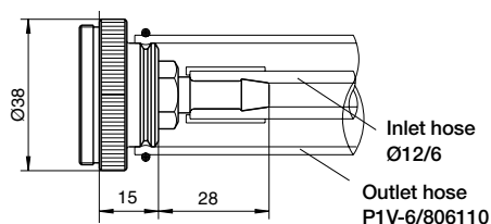
Outlet connection straight P1V-6/313179A
