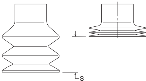
Cup deflection
