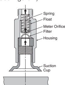
Figure 1 (Closed, Metered Flow)
