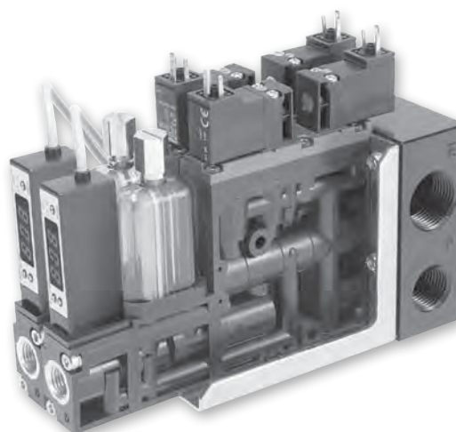
Add-A-Fold assembly (Silencer included)
