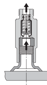
Figure 2 (Open, Full Flow)
