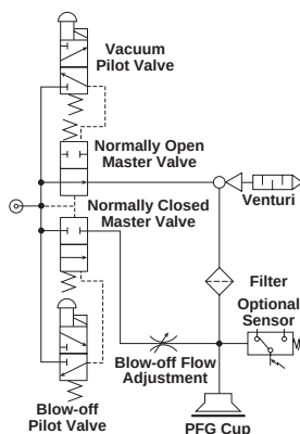
MC22, Normally Open Vacuum Valve
