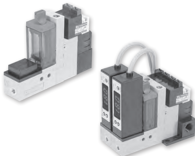
Add-A-Fold Manifold
