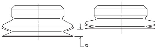
Cup deflection
