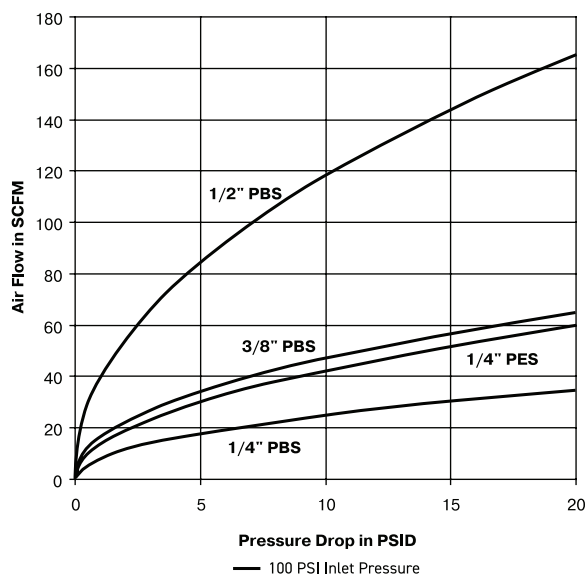
Tool-Mate Series Exhaust (1/4", 3/8" & 1/2" sizes)
