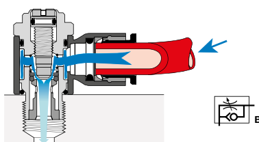
Unidirectional supply model
