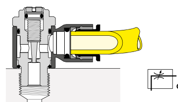
Bidirectional model
