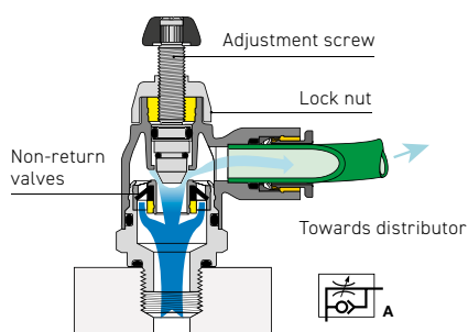
Unidirectional exhaust model
